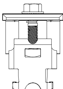
4 4000135 K2 Cross Clamp Set, Mill
